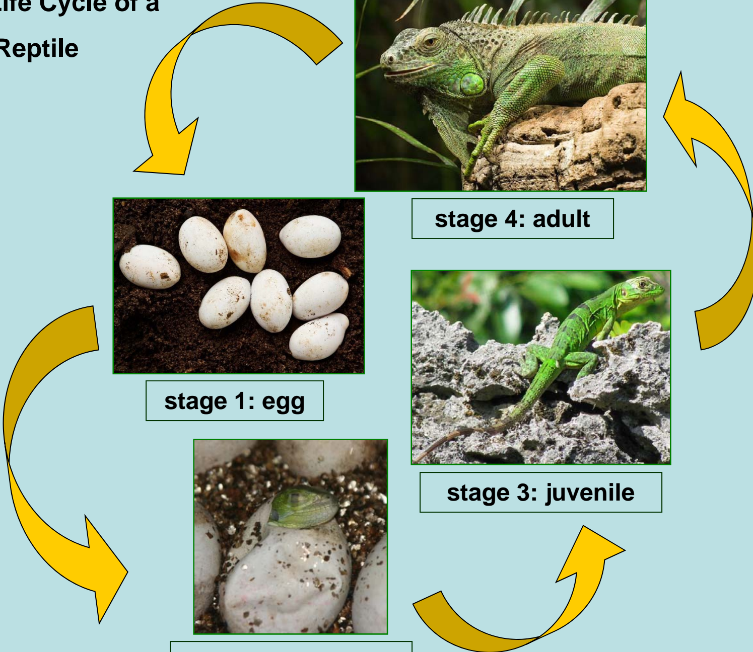
stage 2: hatchling
