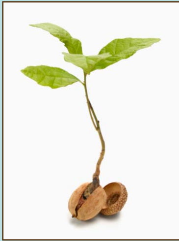
stage 2: seedling
